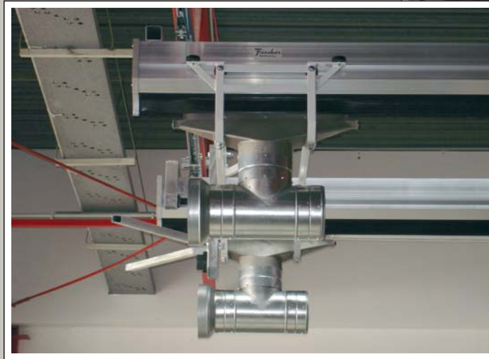
FireMaster Overhead Upward facing exhaust pipes present problems to all exhaust gas extraction systems. But not with our FireMaster Overhead – here is an intelligent solution for every problem.
